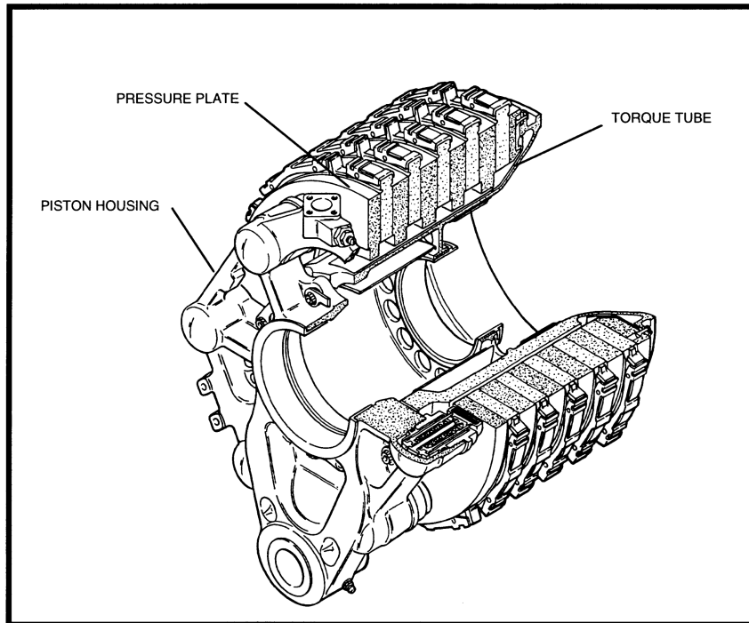
FIGURE 2 - Typical Carbon Heat Sink Brake
